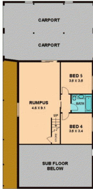
BELOW GROUND
